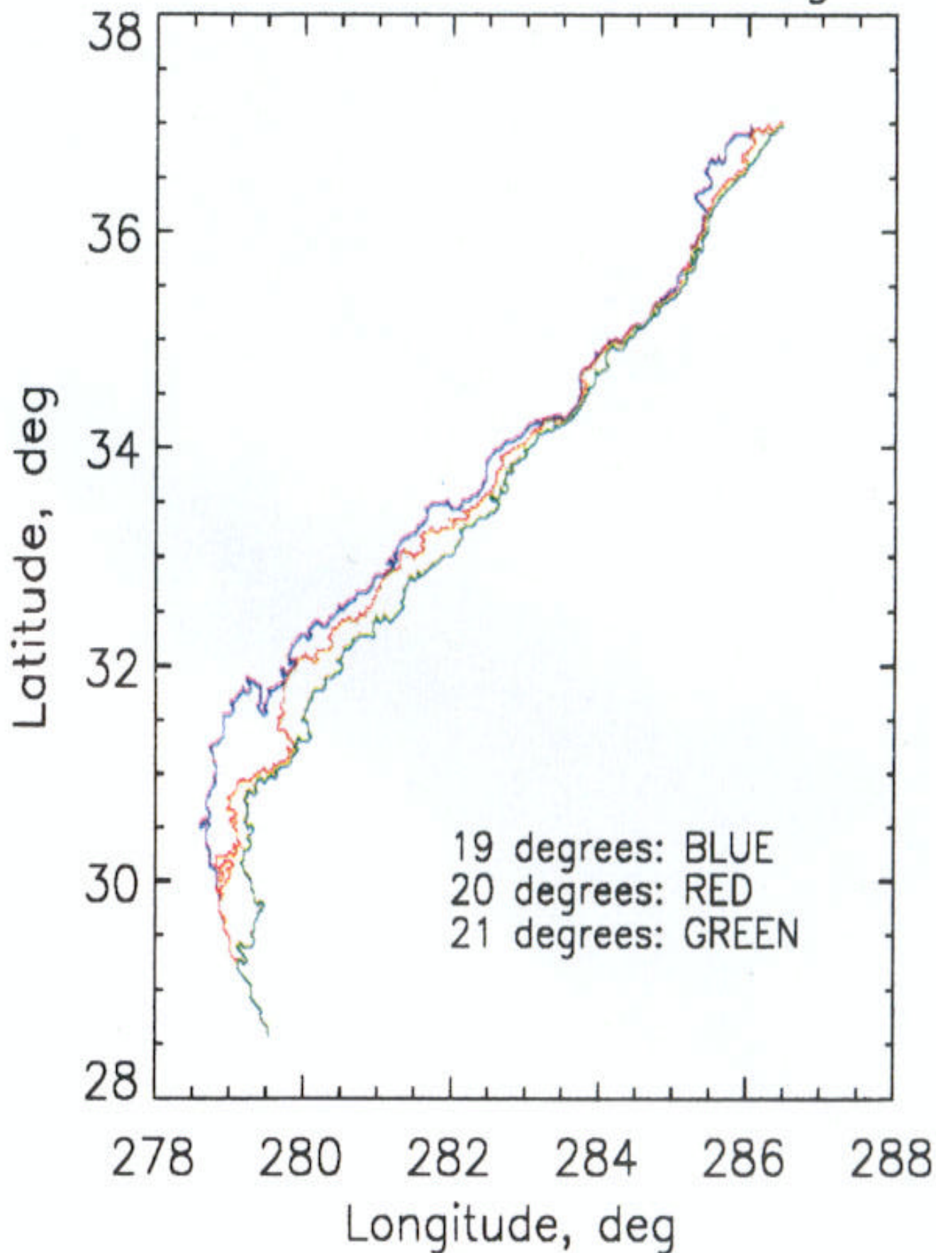
Fig. 4. Temperature fronts less than 37 deg. for image 85.
